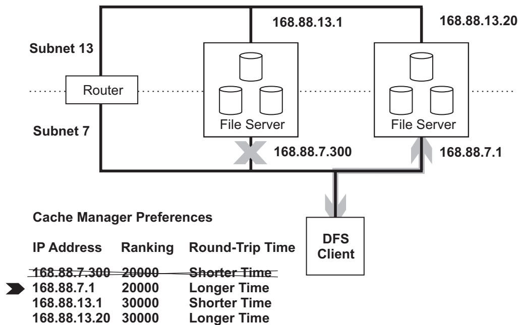
Figure 4. Cache Manager connecting to file server address with next lowest rank
