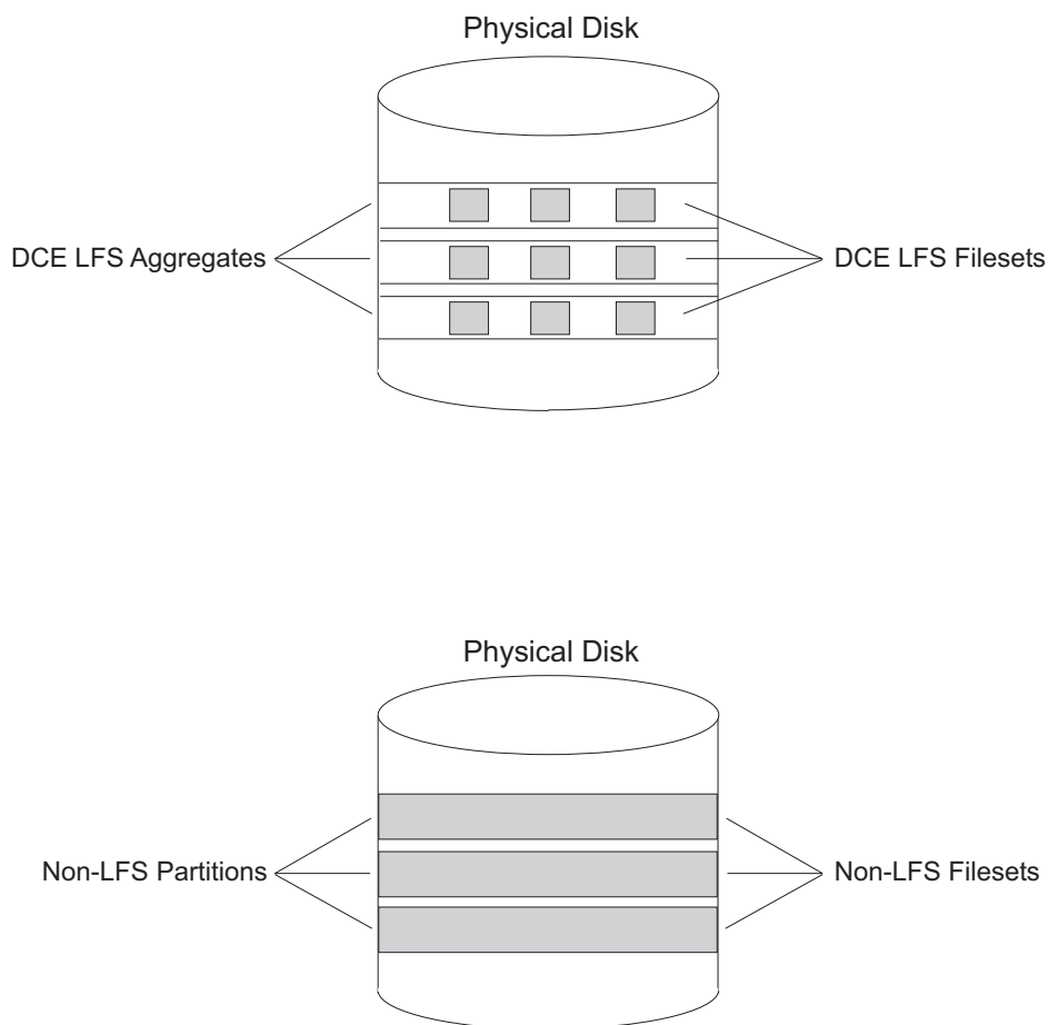
Figure 12. Comparison of DCE Local File System and non-Local File System disk partitioning Structures
