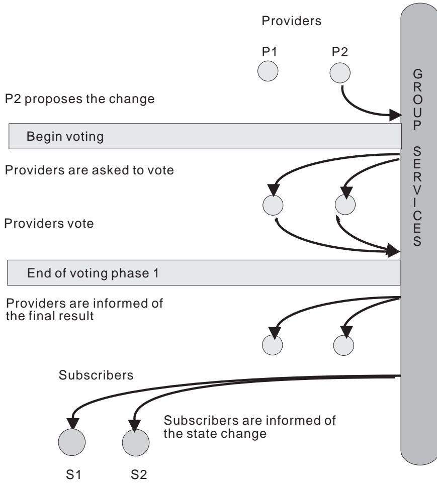
Figure 2. A Two-Phase Commit Protocol
