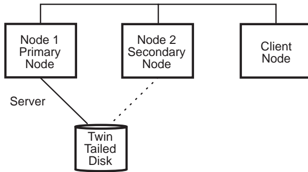
Figure 6. The Primary Node Is the Server Again after Recovery
