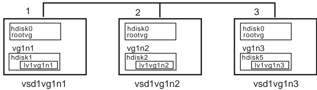
Figure 18. An Example of a Virtual Shared Disk Configuration
