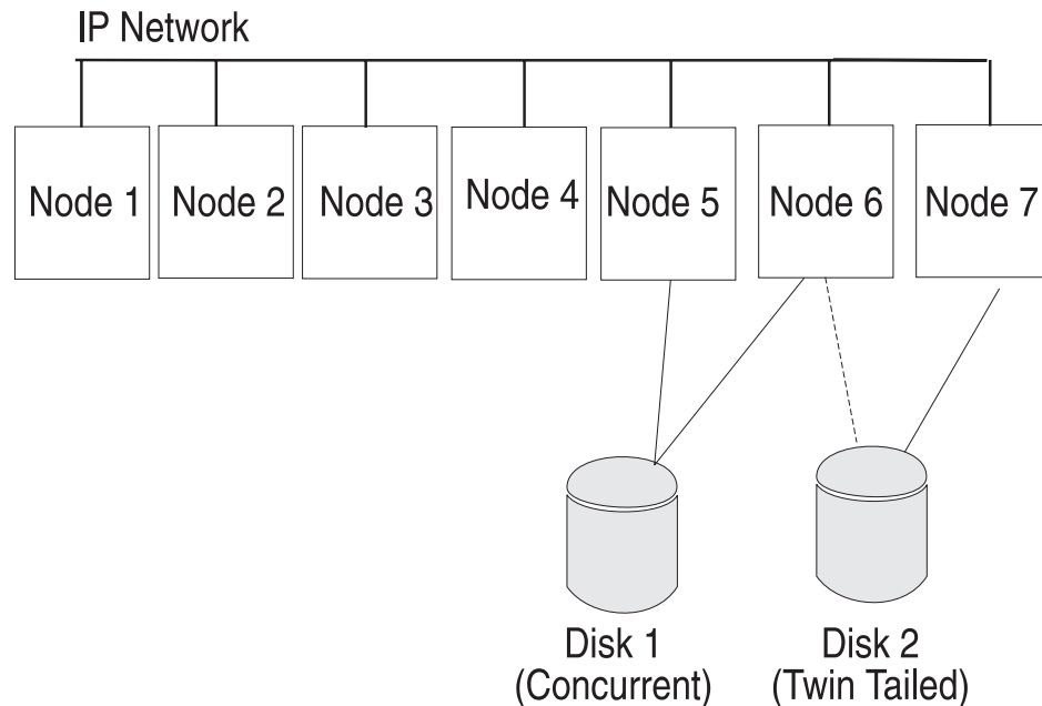
Figure 2. An IBM Concurrent Virtual Shared Disk IP Network Implementation
