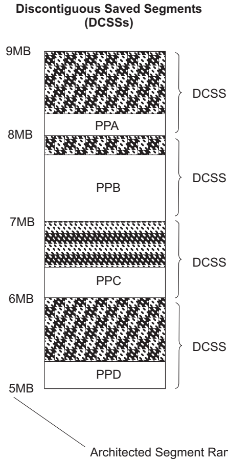
Figure 2. Saved Segments
